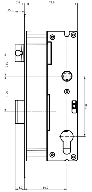
VIRTUS FLUSH MOUNT 2 PT LOCK 60mm BS-13mm DB THROW
