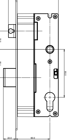
VIRTUS FLUSH MOUNT 2 PT LOCK 60mm BS-22mm DB THROW
