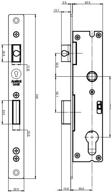
VIRTUS FLUSH MOUNT 2 PT LOCK 30mm BS-13mm DB THROW
