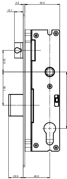
VIRTUS FLUSH MOUNT 2 PT LOCK 40mm BS-22mm DB THROW
