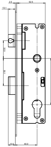
VIRTUS FLUSH MOUNT 2 PT LOCK 40mm BS-13mm DB THROW
