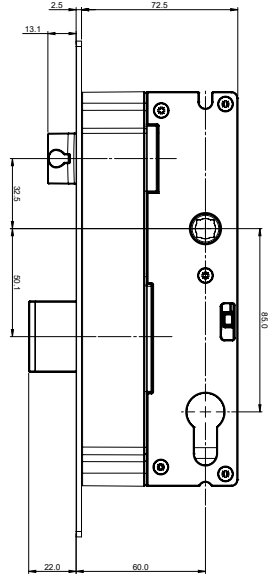
VIRTUS FLUSH MOUNT 2 PT LOCK 60mm BS-22mm DB THROW
