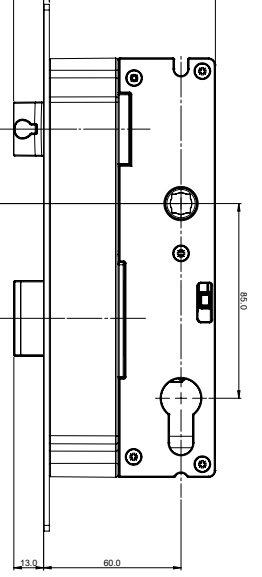
VIRTUS FLUSH MOUNT 2 PT LOCK 60mm BS-13mm DB THROW
